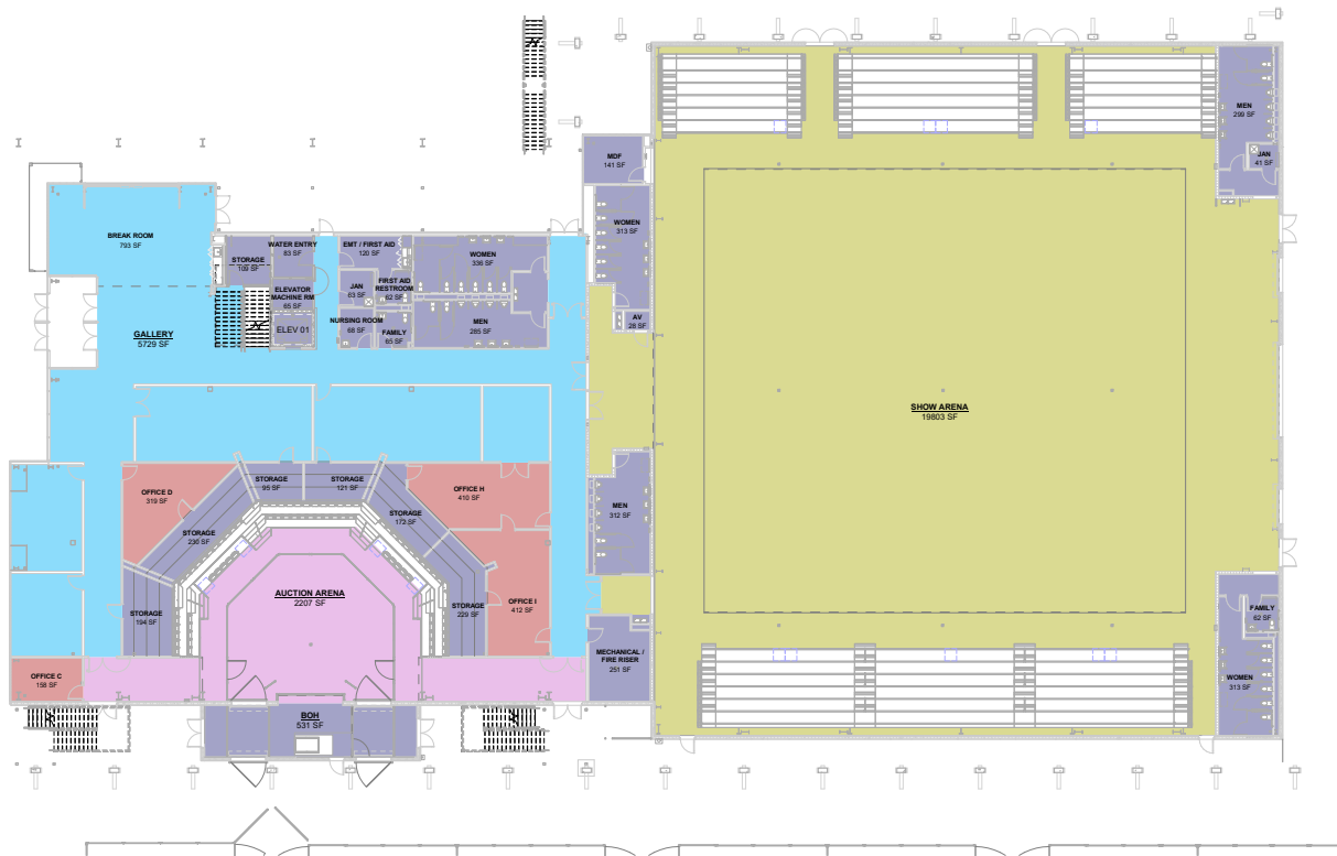
LEVEL 01
